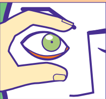
Pin-point pupils
